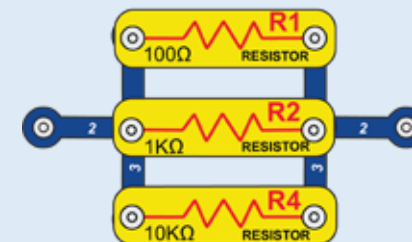
Parallel Circuit
